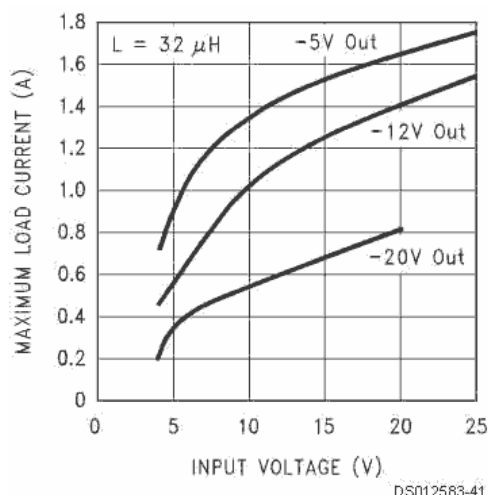
FIGURE 26. Inverting Regulator Typical Load Current
