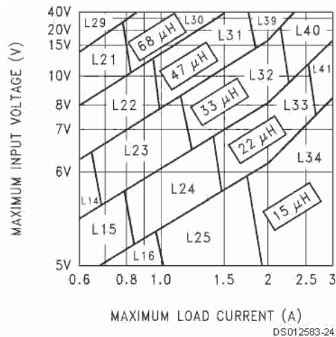
FIGURE 4. LM2596-3.3
