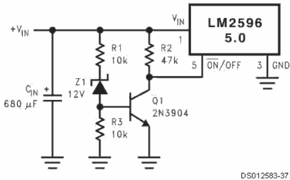
FIGURE 22. Under voltage Lockout for Buck Regulator DELAYED STARTUP
