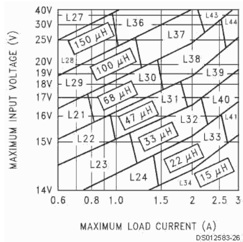
FIGURE 6. LM2596-12
