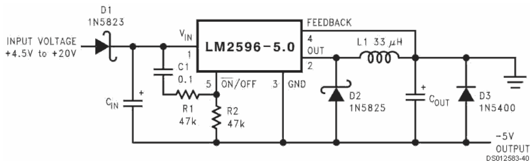
FIGURE 24. Undervoltage Lockout with Hysteresis for Inverting Regulator
