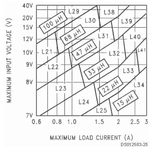
FIGURE 5. LM2596-5.0
