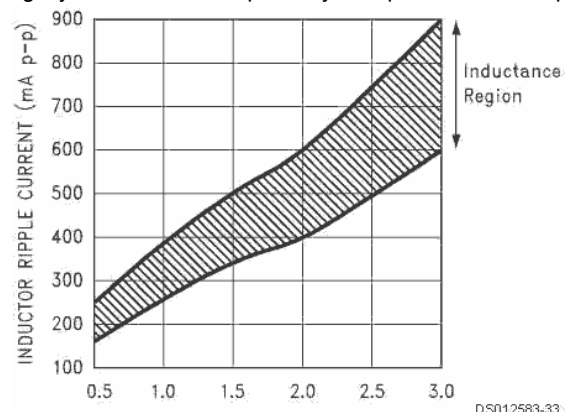
FIGURE 18. Peak-to-Peak Inductor Ripple Current vs Load Current In a switching regulator design, knowing the value of the
