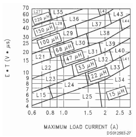
FIGURE 7. LM2596-ADJ
