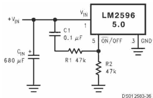
Figure 21. Delayed Startup
